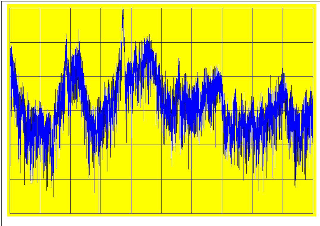
Toxin architecture: high hollow peak
